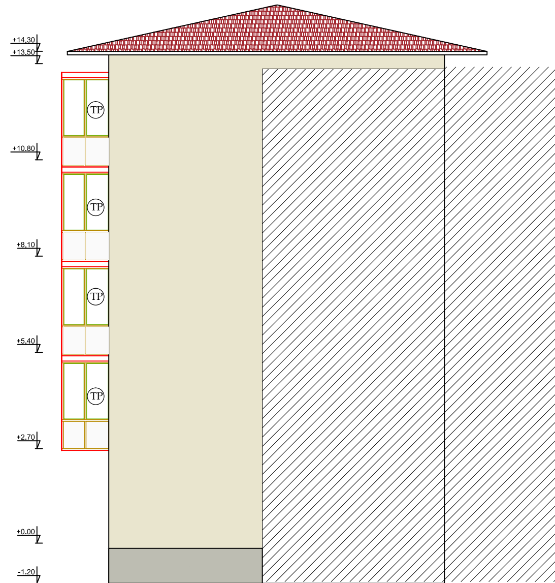
Fatada laterala stanga propusa
